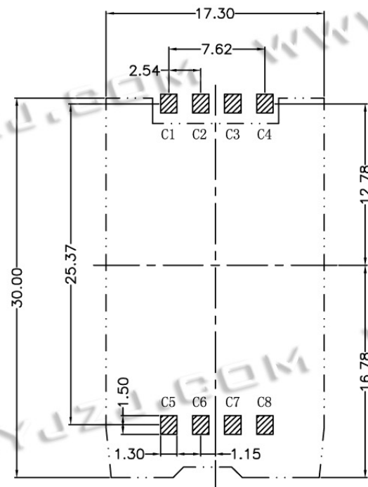
RECOMMENDED P.C.B LAYOUT COMPONENT SIDE (TOLERANCE \pm 0.05 )
